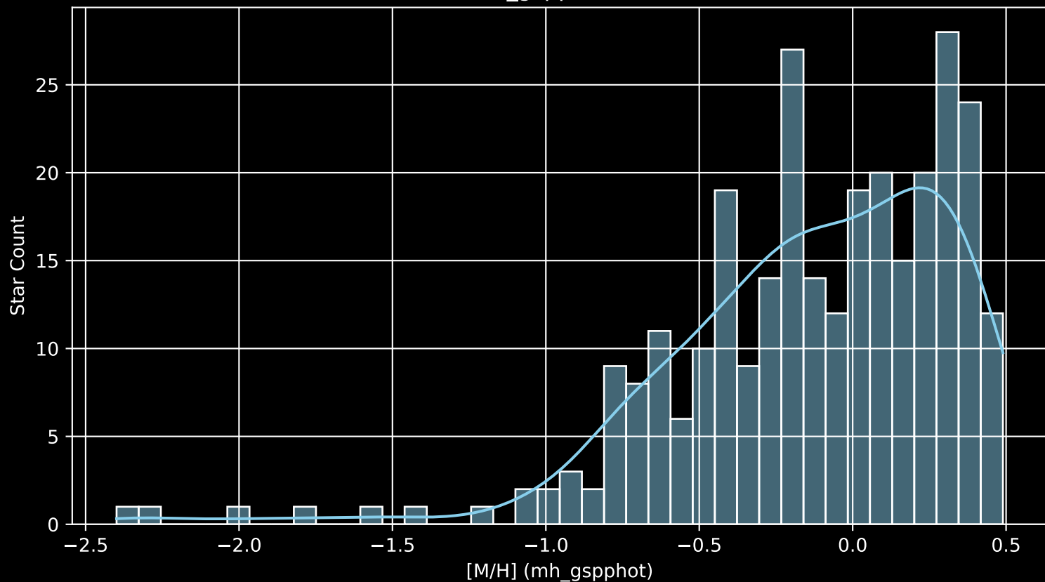
APOGEE DR17 Field: [030+04 [M/H] (mh_gspphot) (n= 293)
