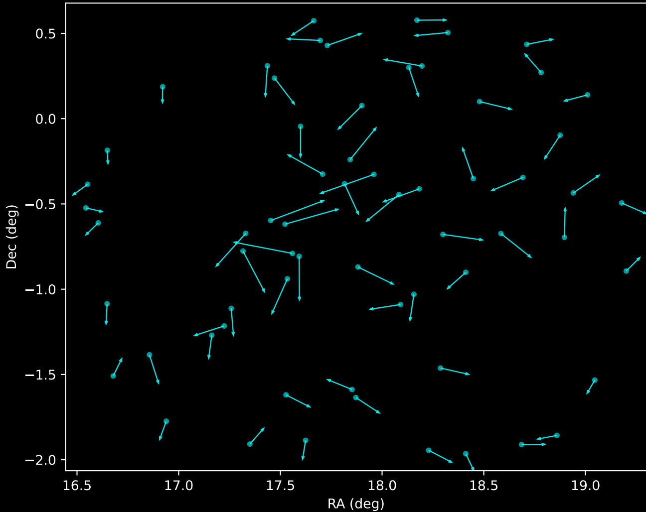
APOGEE DR17 Noise Stream Proper Motion Vectors (n=64)
