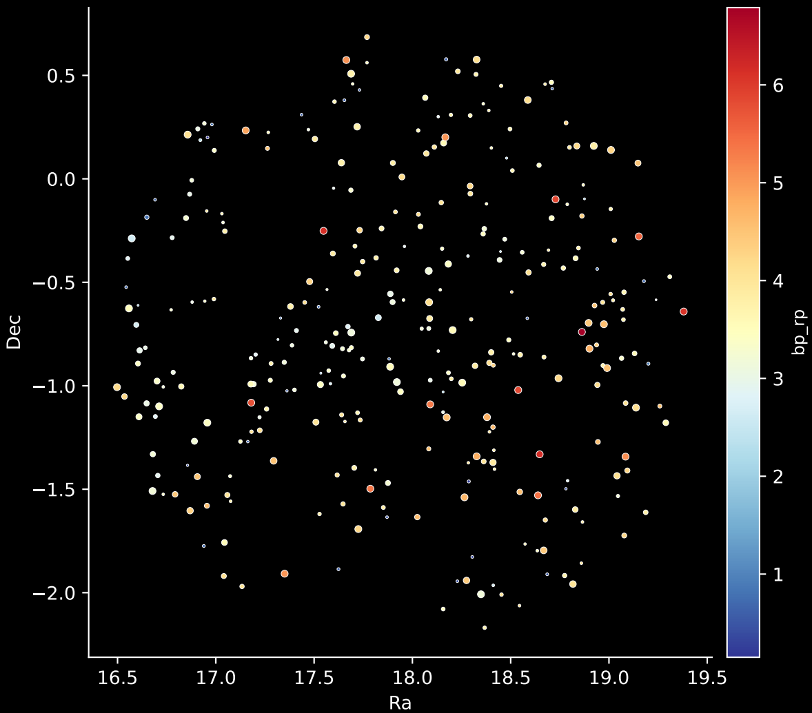
APOGEE DR17 Field: [030+04] Stars: 315
