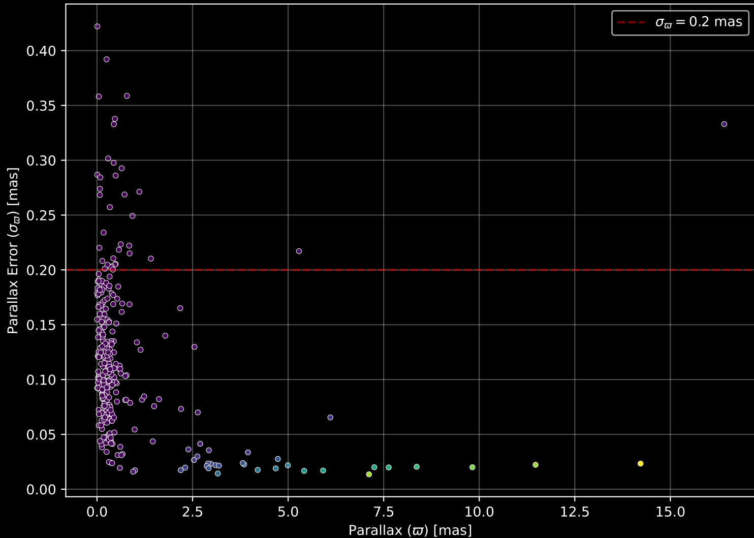
APOGEE DR17 Field: [030+04] Parallax Quality (n= 315)
